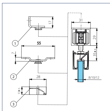
Rollan with glass clamping plate 30 mm
