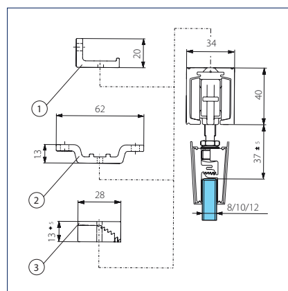
Perlan with glass clamping plate 45 mm
