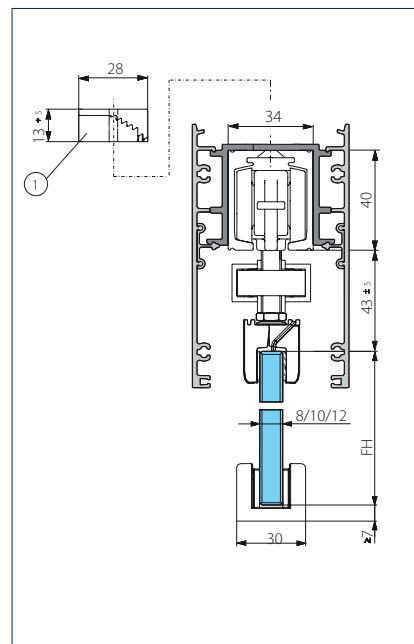
Wall / ceiling mounting glass with glass clamping plate 30 and clip-on cover 100 on both sides
