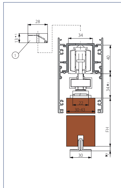
Wall / ceiling mounting wood with clip-on cover 100 on both sides
