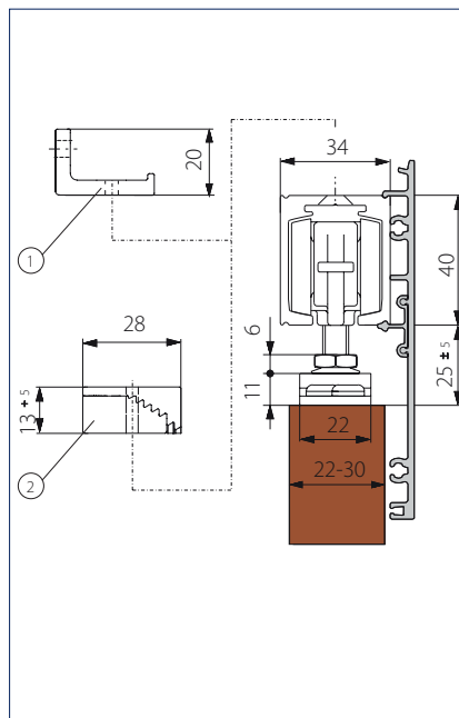
Wall / ceiling mounting glass with clip-on cover 100
