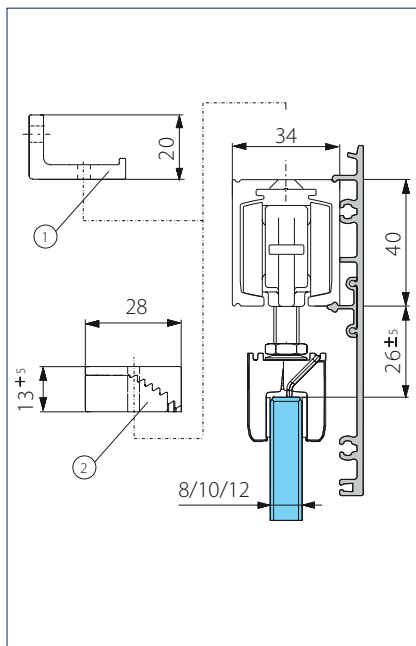
Wall / ceiling mounting glass with glass clamping plate 30 and clip-on cover 100
