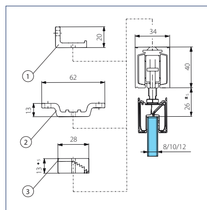
Perlan with glass clamping plate 30 mm
