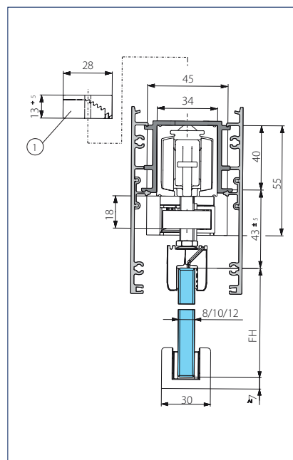
Wall / ceiling mounting glass with clip-on cover 100, on both sides
