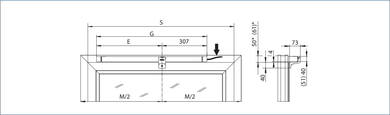
See table for dimensions for E, G and S Dimensions in brackets apply for side-hung windows DIN left I * = Swivelling range
